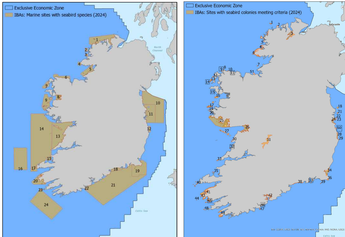
Left panel: New marine sites. Right panel: New (in black squares) and reassessed terrestrial sites.
