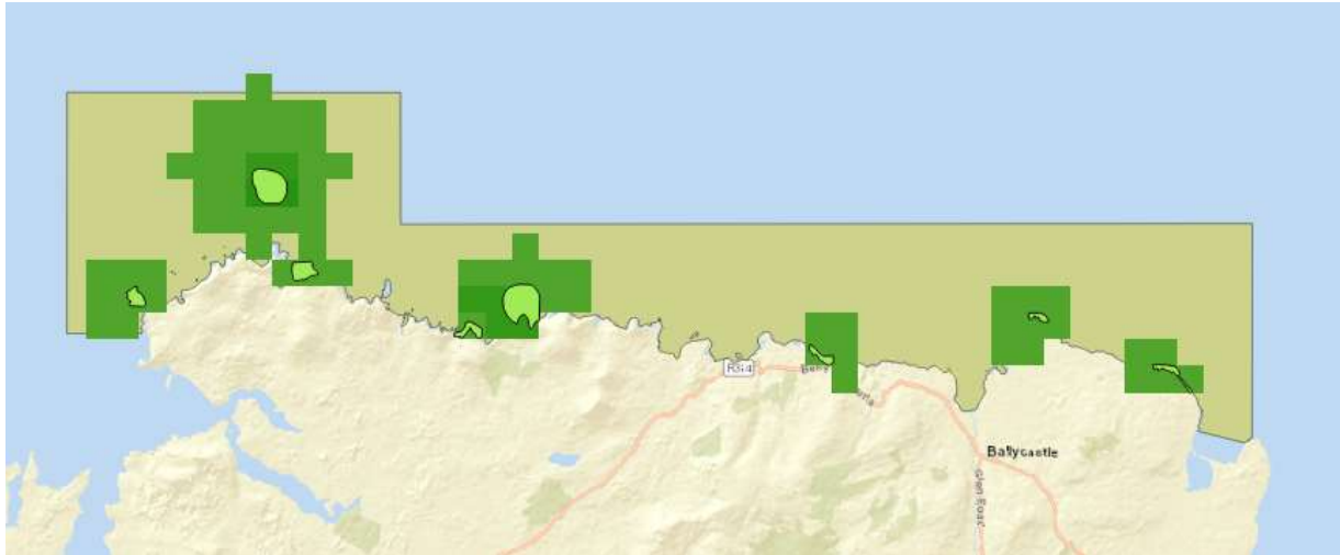
Figure 14: The North Mayo coast and islands marine extension site considerations. See text for full explanation.
