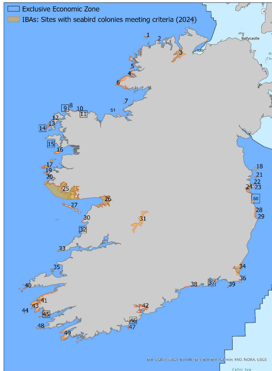
Figure 5: Colonies: Sites with seabird colonies meeting criteria (9 new sites shown with black outline)
