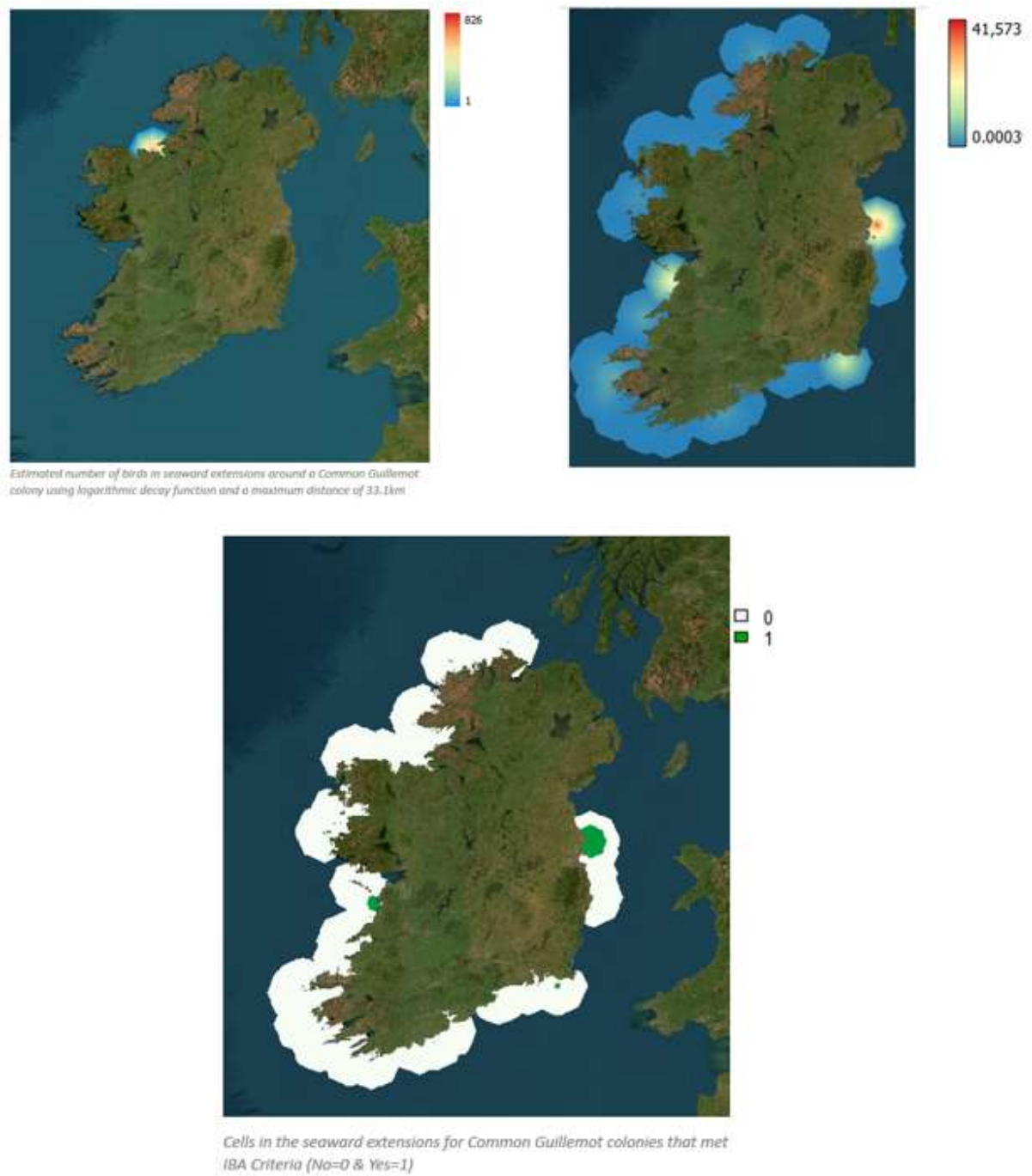
Figure 16: Example of decay function estimate of at-sea distribution around breeding locations for Common Guillemot, with final sites meeting criteria indicated in the bottom panel.
