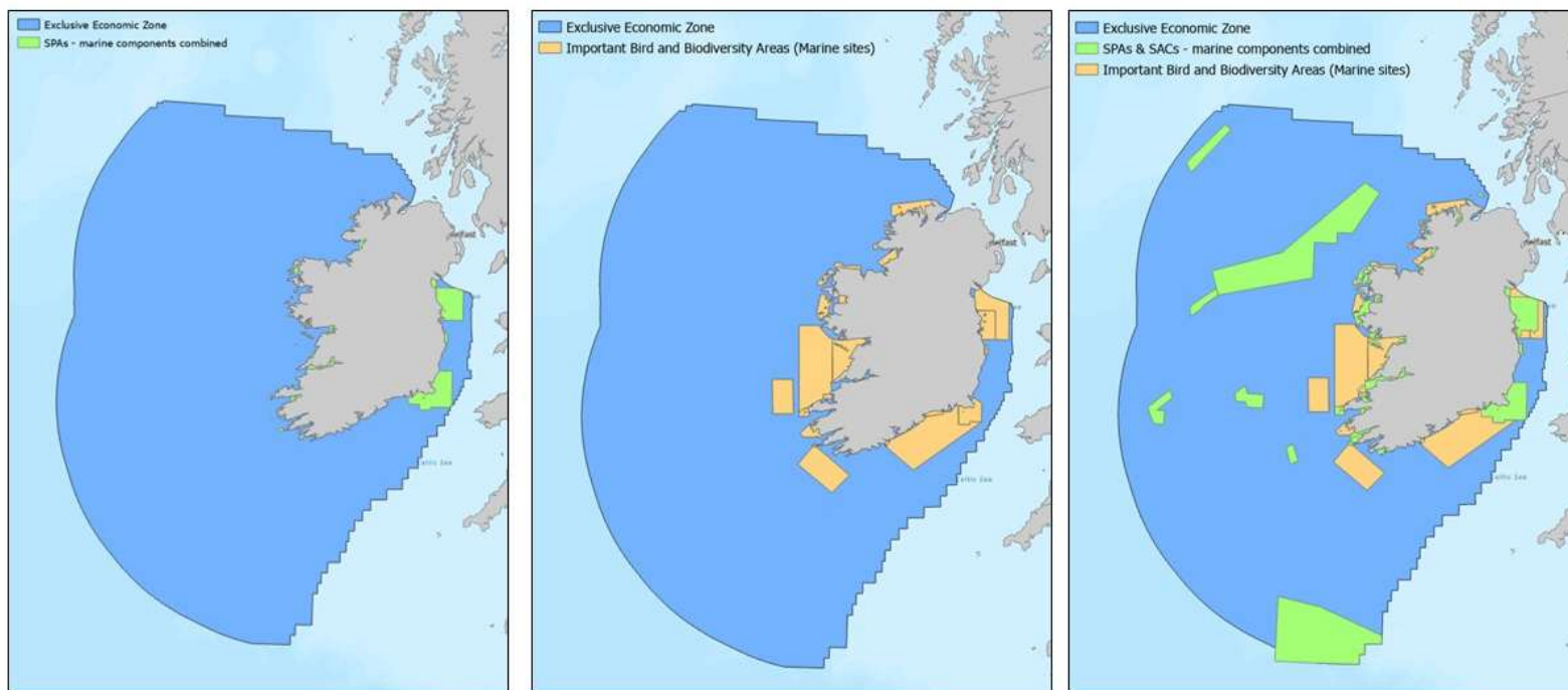
Figure 7: Ireland's EEZ showing marine cSPAs (L), marine IBAs (middle) and all marine Natura sites with IBAs (R)
